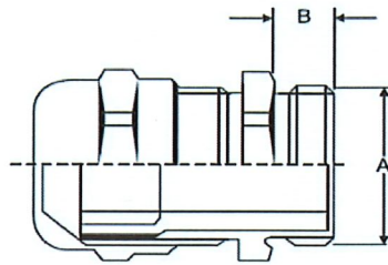
Plated Brass Gland - IP68 Rating - Metric Thread
